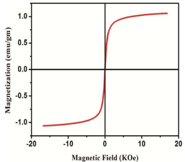
Fig. 4 — Magnetic hysteresis loop for \gamma -Fe 2 O 3 nanoparticles
