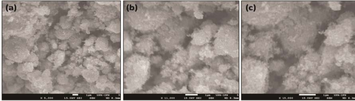
Fig. 2 — Scanning electron microscopy (SEM) images of \gamma -Fe 2 O 3 nanoparticles at different magnifications (a) 5000X (b) 11000X (c) 15000X
