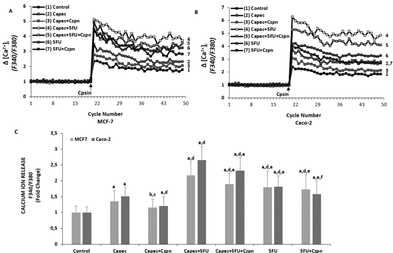
Fig. 1 — In vitro effect of Capecitabine (2 \mu M, 24 h) and 5FU (2,5 \mu M, 24 h) on the free intracellular calcium increase ( [Ca^{2+}]_i ) through TRPV1 channels in MCF-7 (A) and Caco-2 (B) cells and cellular calcium ion release (C). (n=3 and mean \pm SD). The cells are stimulated by capsaicin (Cpsin and 0.1 mM on the 20 th cycle) but they were inhibited by capsazepine (Czpn and 0.1 mM for 30 min). a P < 0.001 and b P < 0.05 vs control, c P < 0.05 , and d P < 0.001 vs Capec, e P < 0.001 vs Capec+5FU, f P < 0.001 vs 5FU
