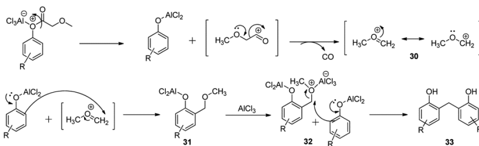
Scheme V — Plausible mechanism for the synthesis of methylene-bis-compounds
