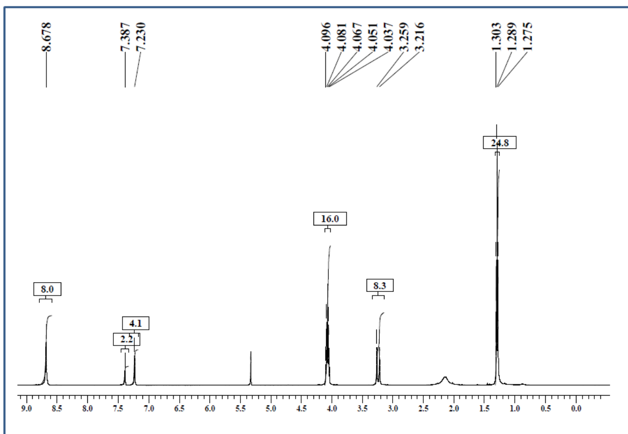
Figure S1- 1 H NMR spectra of compound 3.
