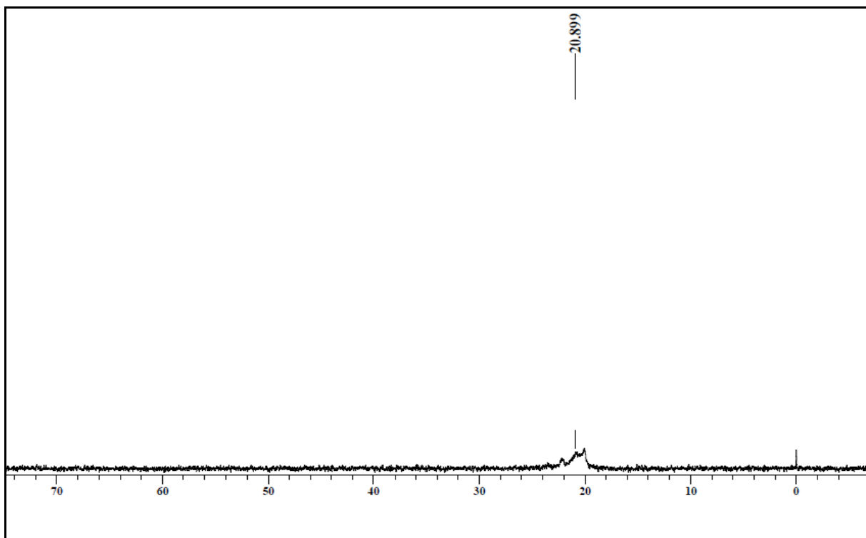
Figure S8 - 31 P NMR spectra of compound PDI-TPA .
