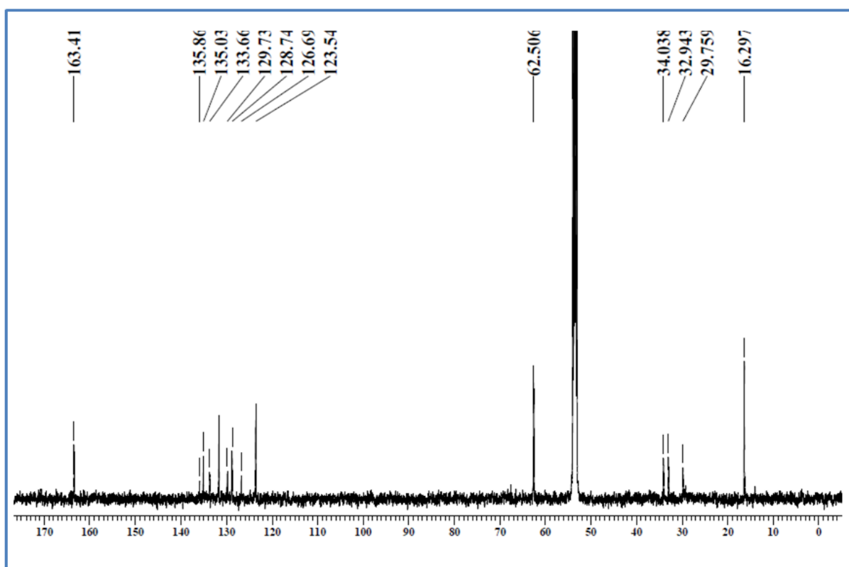
Figure S2 - ^{13}\text{C} NMR spectra of compound 3.
