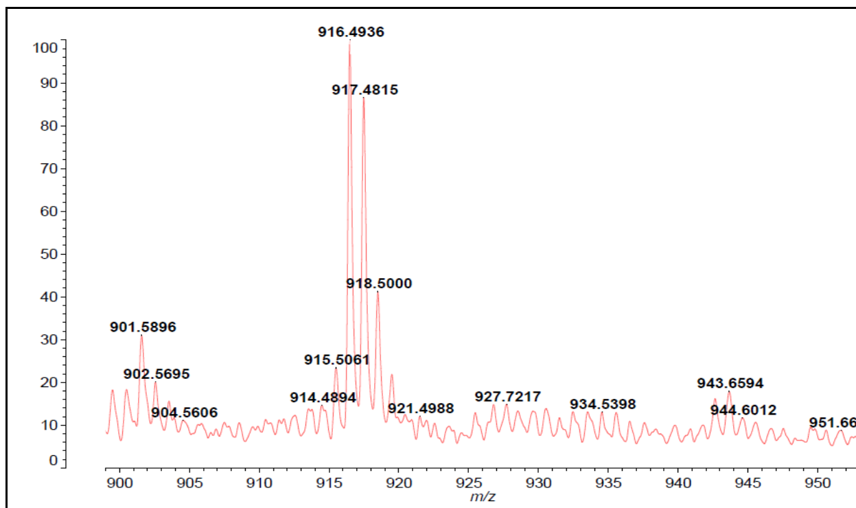
Figure S9 -MALDI-TOF spectrum of compound PDI-TPA .
