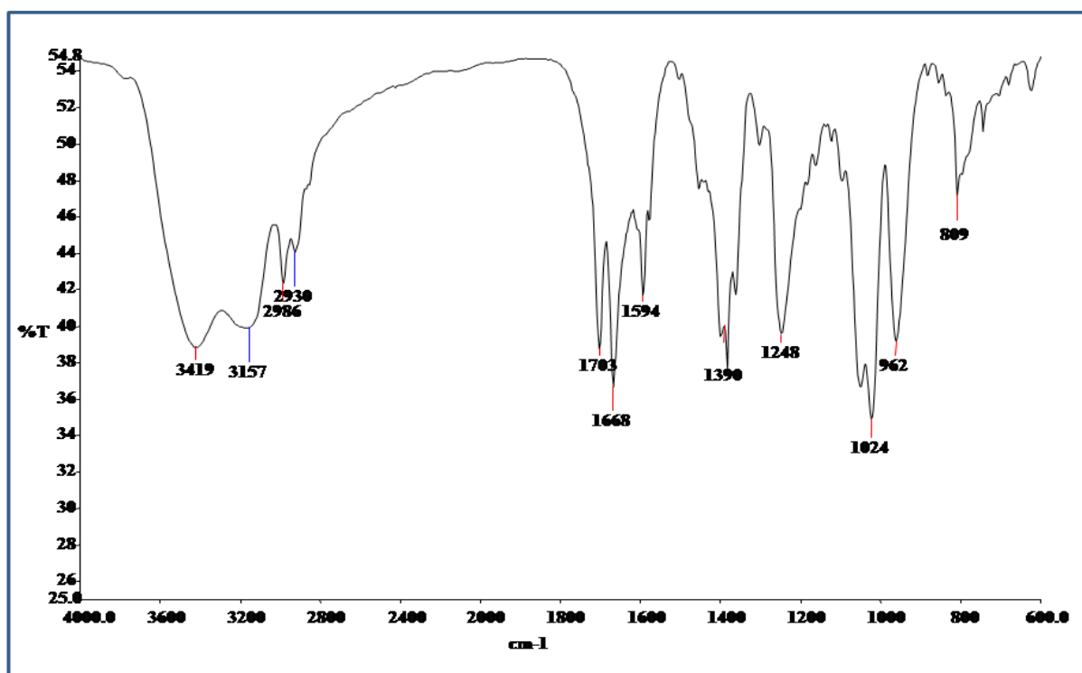
Figure S6- FT-IR spectra of compound 3.
