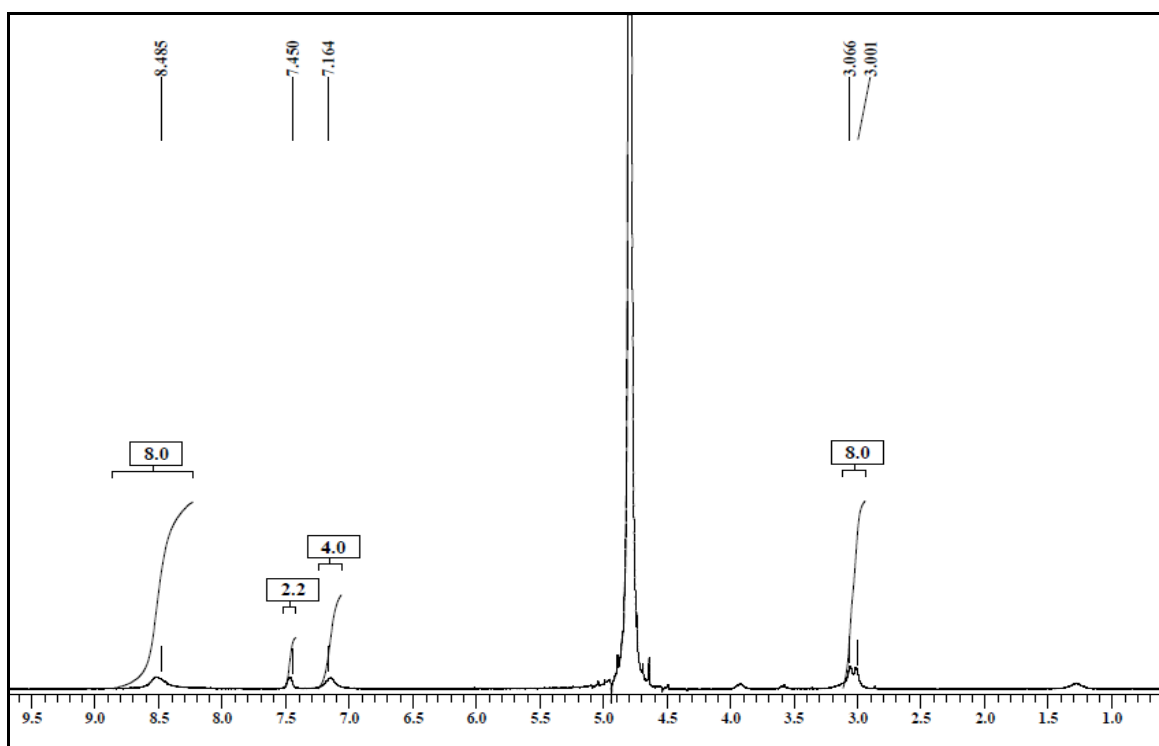
Figure S7 - 1 H NMR spectra of compound PDI-TPA.
