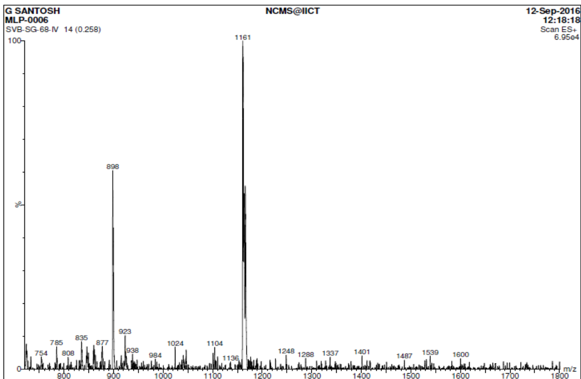
Figure S4 -ESI-Massspectrum of compound 3.
