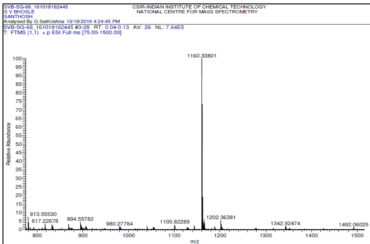
Figure S5 -HRMS spectrum of compound 3.
