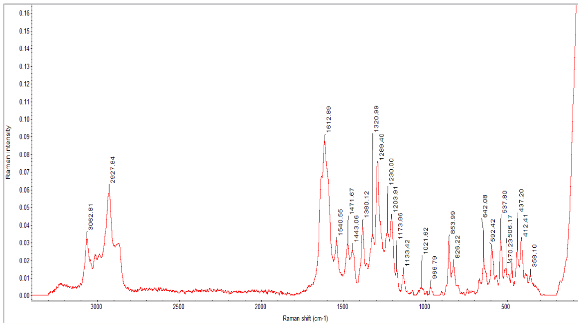
Fig 5. Micro-Raman
