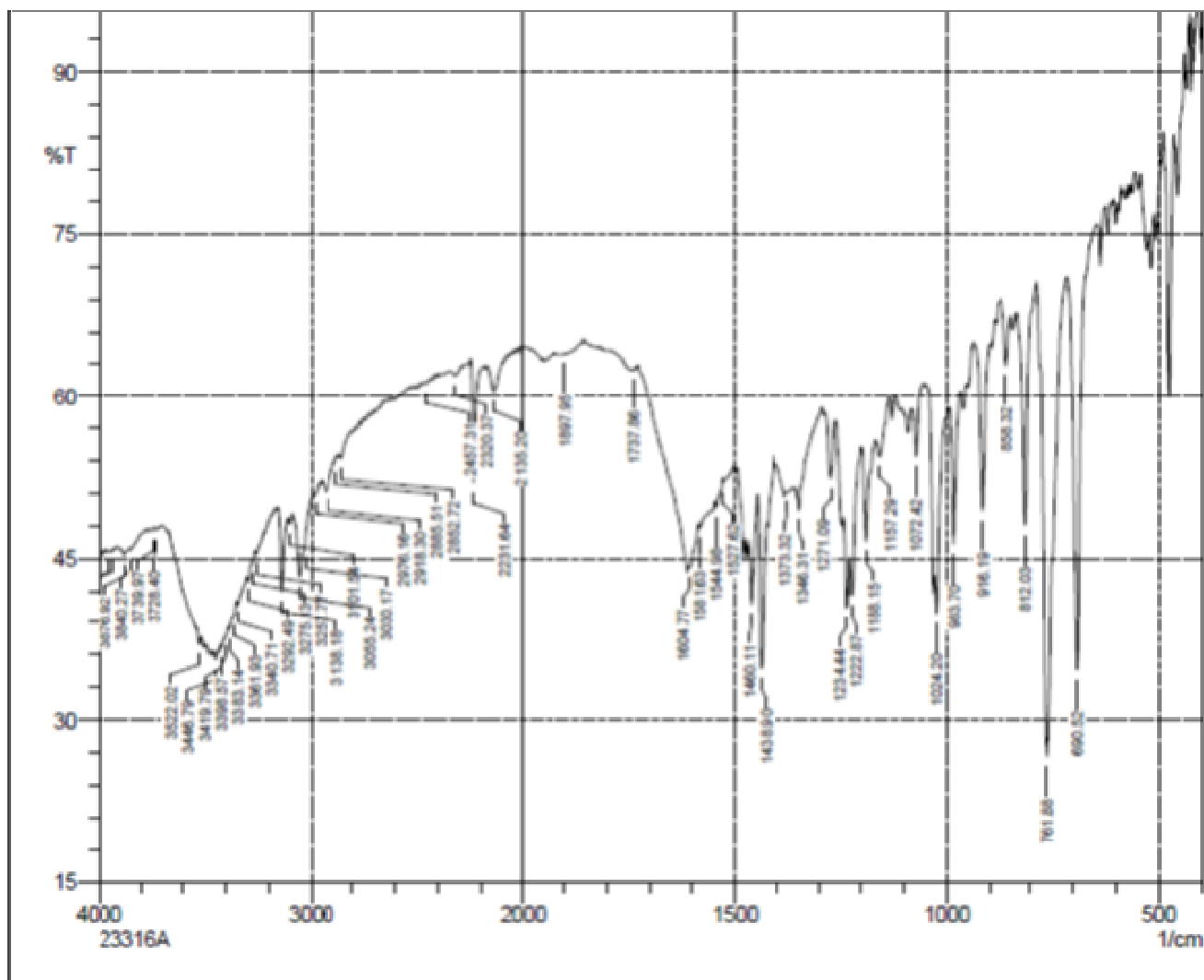
Fig.S17: IR spectrum of 2-(4-Phenyl-[1,2,3]triazol-1-yl)-benzo[f]chromen-3-ylideneamine 6a
