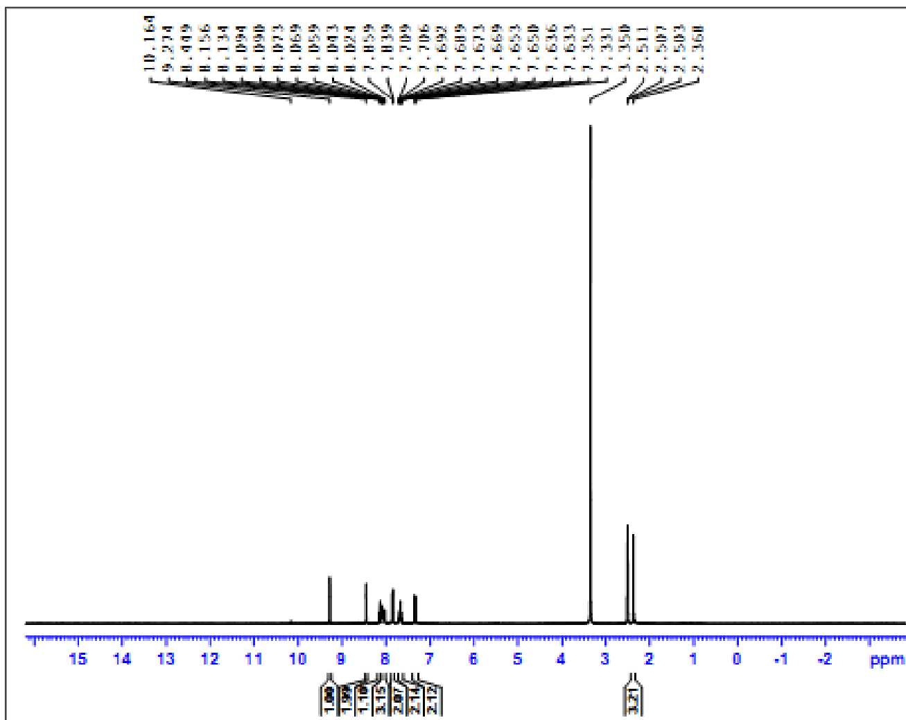
Fig.S18: 1 H NMR spectrum of 2-[4-(4-methylphenyl)1H-[1,2,3]triazol-1-yl)-3H-benzo[f]chromen-3-ylideneamine 6b
