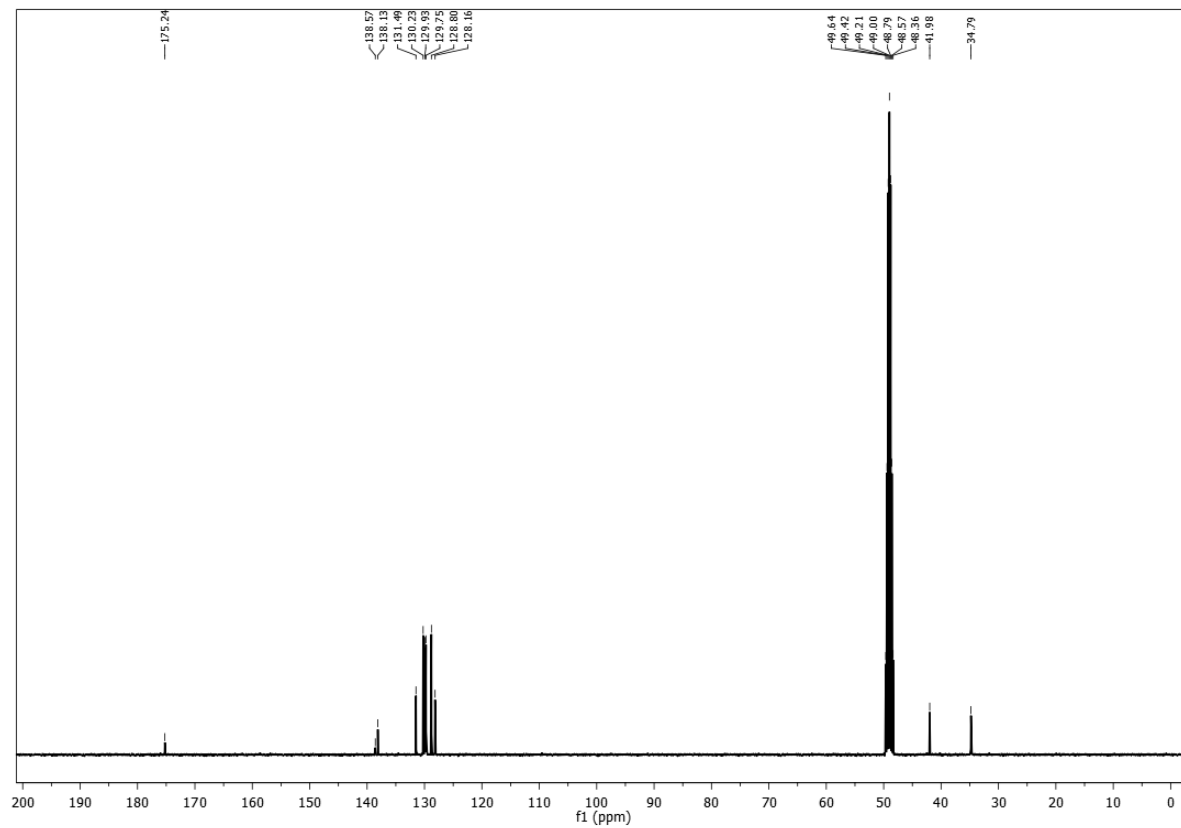
Fig. S10 — ^{13}\text{C} NMR spectrum of 2
