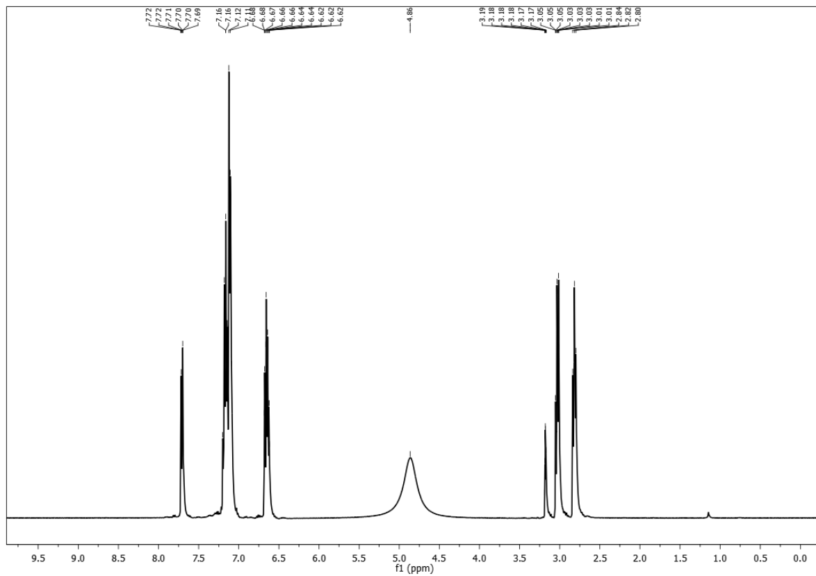
Fig. S7 — ^1\text{H} NMR spectrum of 3
