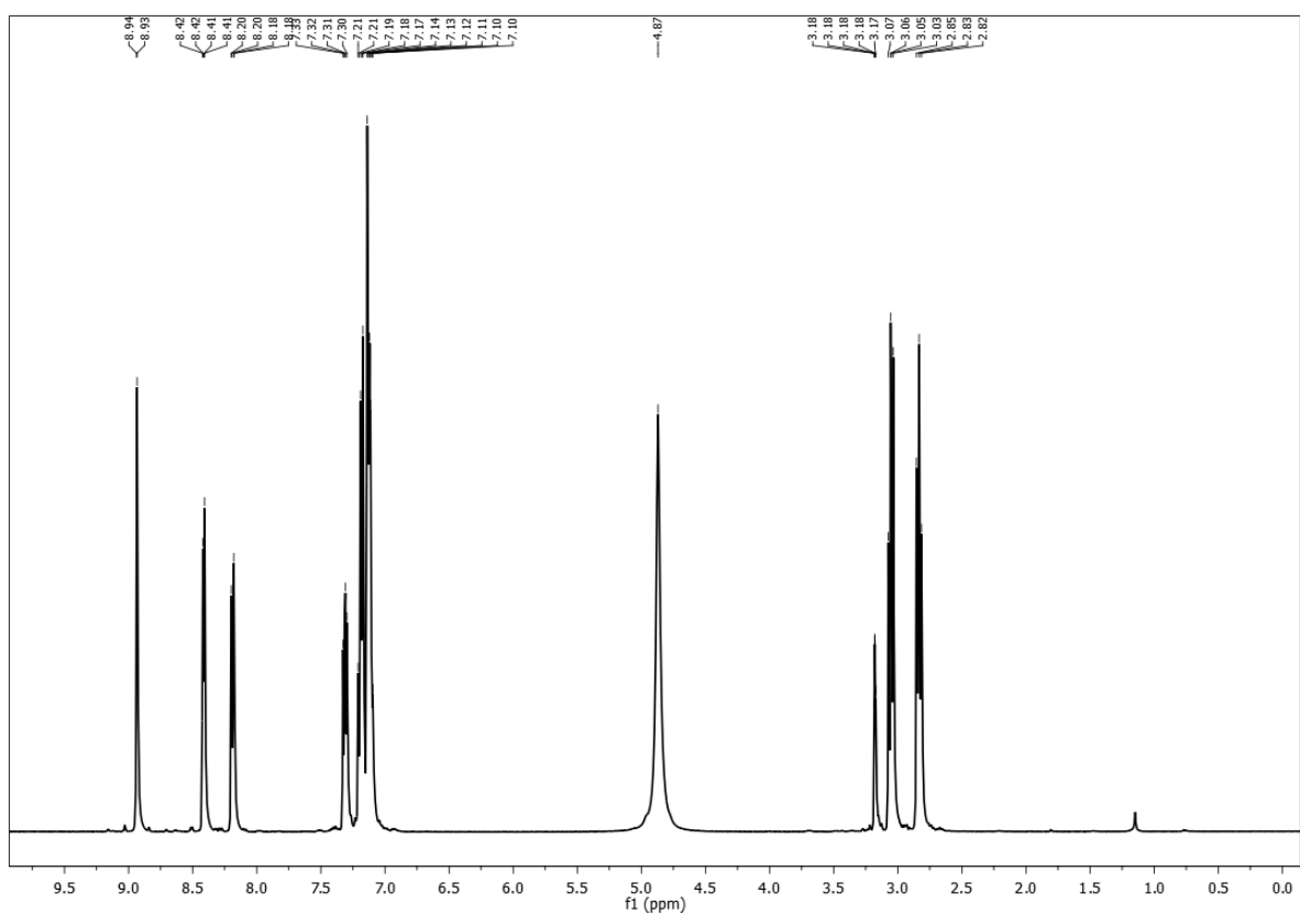
Fig. S5 — ^1\text{H} NMR spectrum of 1
