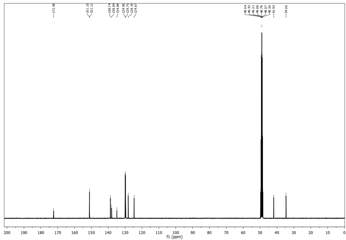
Fig. S9 — ^{13}\text{C} NMR spectrum of 1
