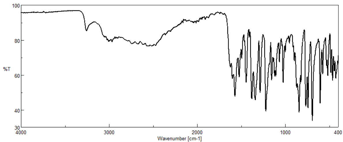
Fig. S4 — FTIR spectrum of 4
