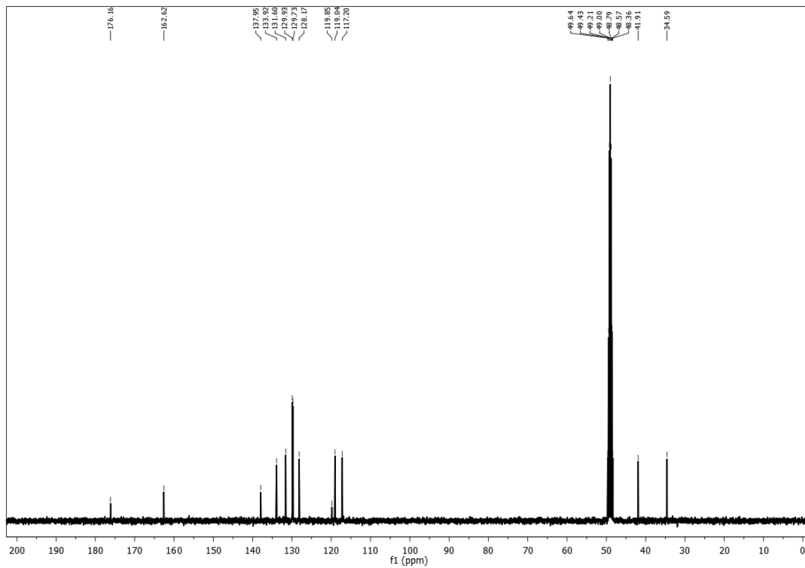
Fig. S11 — ^{13}\text{C} NMR spectrum of 4
