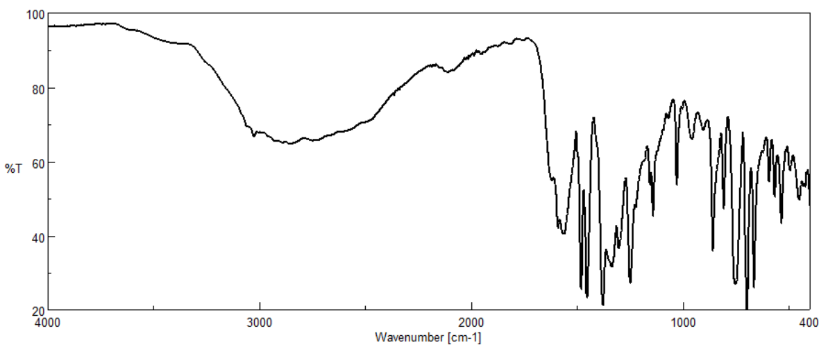
Fig. S3 — FTIR spectrum of 3
