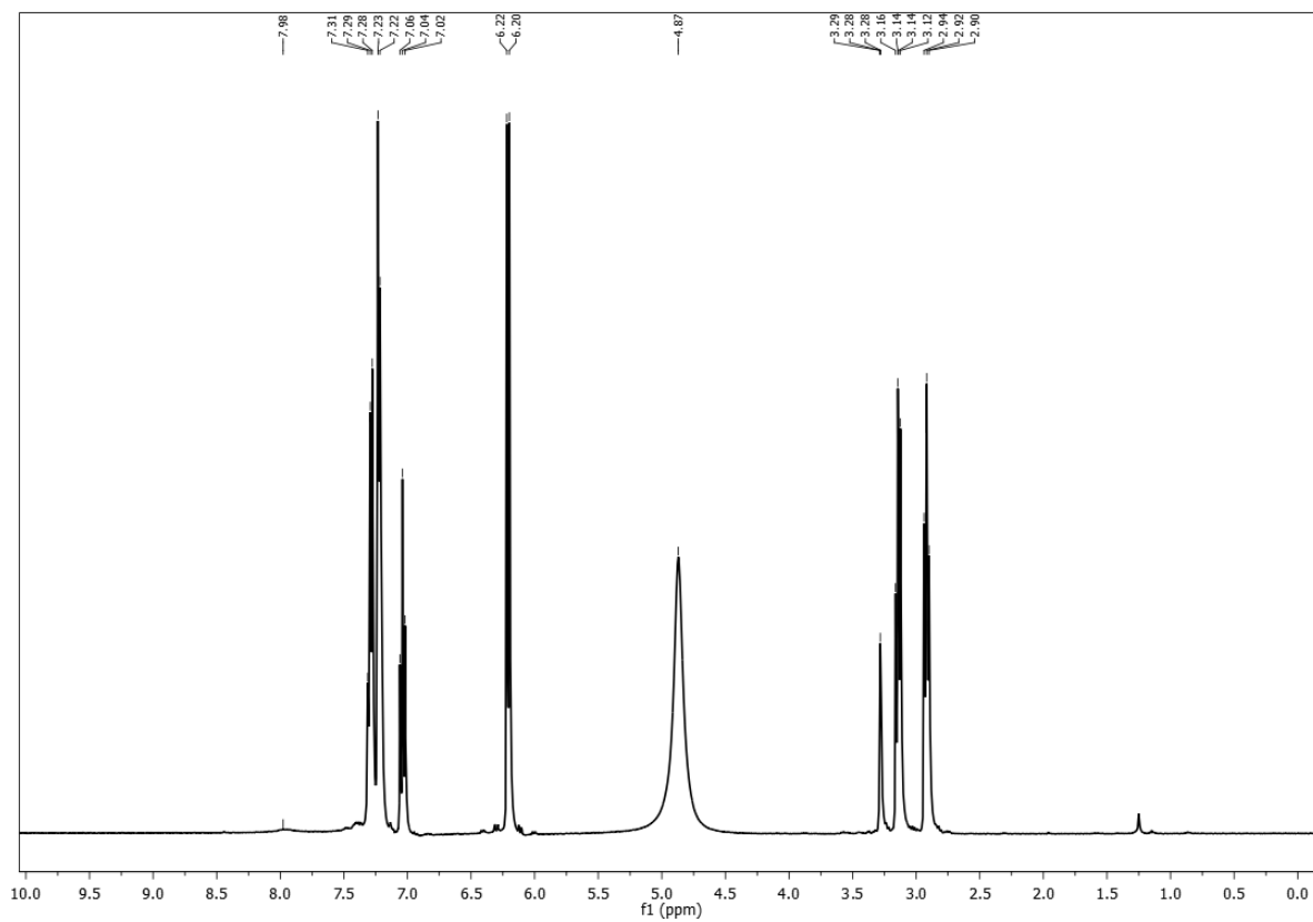
Fig. S8 — ^1\text{H} NMR spectrum of 4
