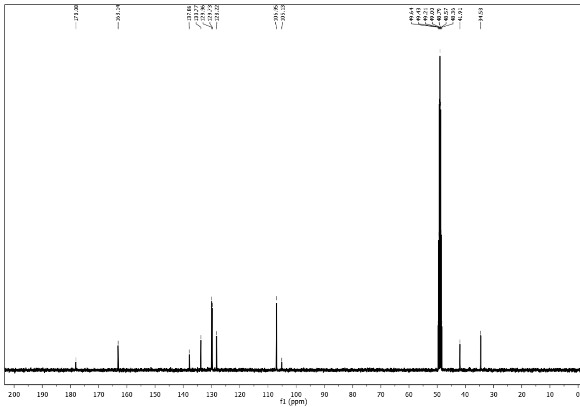
Fig. S12 — ^{13}\text{C} NMR spectrum of 4
