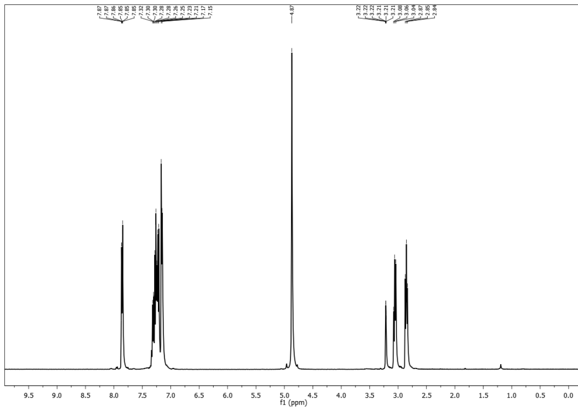
Fig. S6 — ^1\text{H} NMR spectrum of 2
