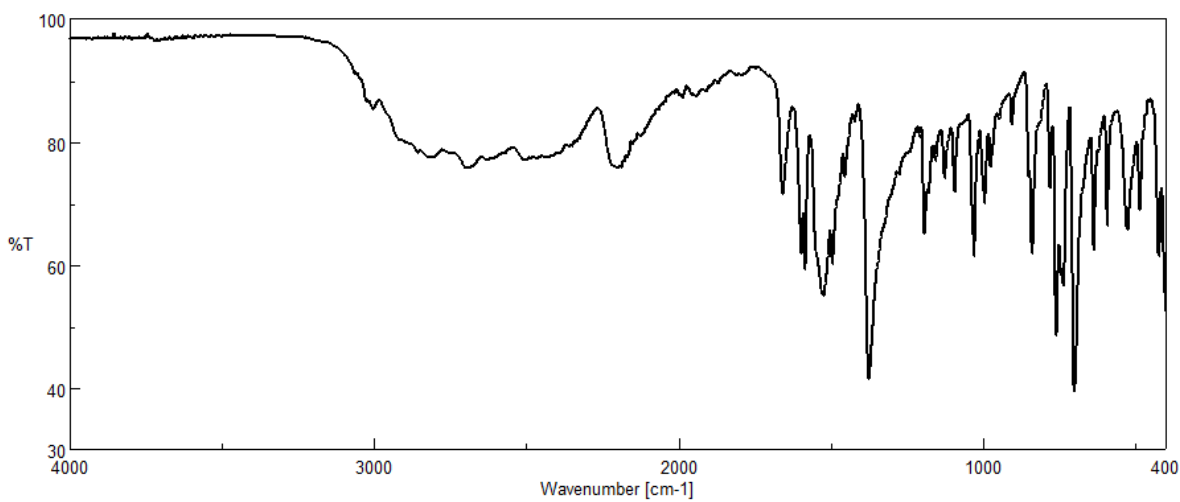
Fig. S1 — FTIR spectrum of 1
