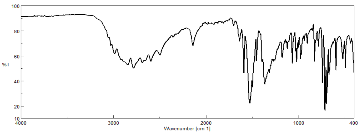
Fig. S2 — FTIR spectrum of 2
