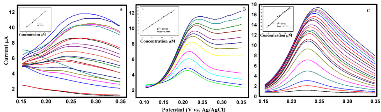
Fig. 5 — DPV of oxidation of DH in 0.1M PBS with (A) GCE-TCP (B) GCE-TCP/FC and (C) GCE-TCP/FC/AuNPs at different concentrations of DH in 0.1 M PBS at a scan rate of 50\text{mVs}^{-1} (Inset: Calibration plot for concentration of DH vs. Current)
