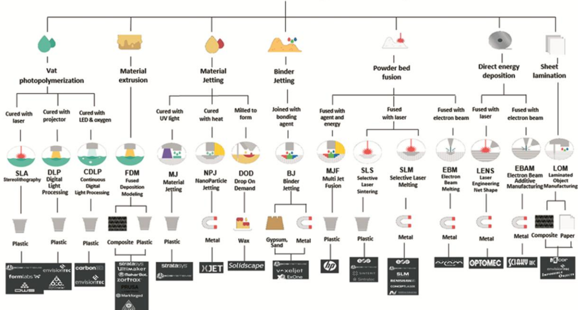
Fig. 1 — Scheme of all additive manufacturing technologies 2 .
