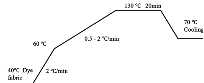
Fig. 1—Dyeing curve for PTT/PET bi-component filament fabrics
