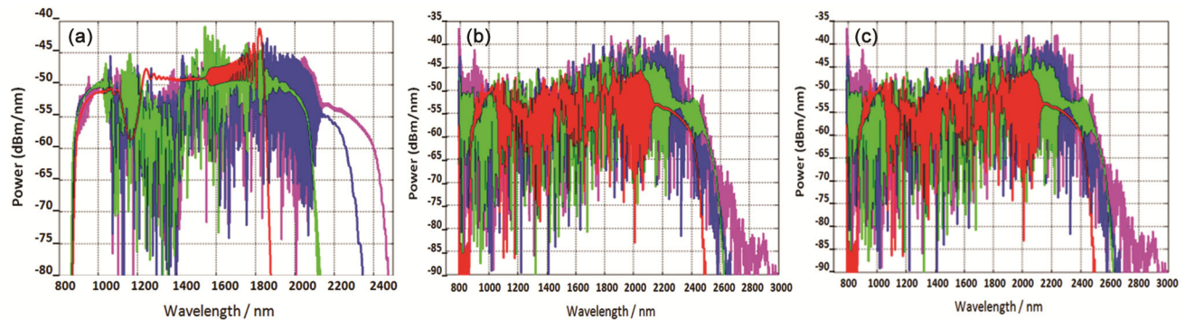
Fig. 9 — Supercontinuum spectrum of PCFS 2,0,3 simulated for length 1cm (red), 4cm (green), 7cm (blue) and 10cm (magenta) with pump energy E = 2\text{nJ} , width T = 350\text{fs} (a); for length 10cm, with pump energy 2nJ and width T = 50\text{fs} (magenta), 150 fs (green), 250fs (blue) and 350fs (red) (b); and for length 10cm with pump width T = 350\text{fs} and energy E = 2\text{nJ} (red), 4nJ (green), 6nJ (blue) and 8nJ (magenta) (c).
