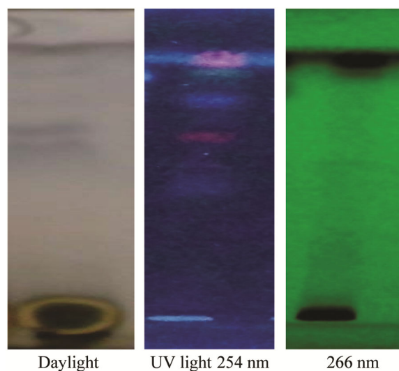
Daylight UV light 254 nm 266 nm Solvents — Benzene: Ethyl Acetate (8:2) Benzene: Ethyl Acetate (8:2) Fig. 1 — TLC pictures showing spot in daylight and UV light at wavelength 254 and 266 nm
