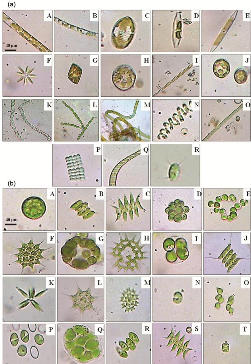
Fig. 2(A) — Microphotographs of phytoplankton belonging to Bacillariophyceae (A-J) (A) Leptocylindrus danicus (B) Aulacoseira sp. (C) Navicula sp. (D) Nitzschia sp. (E) Fragilaria sp. (F) Nitzschia holsatica (G) Cyclotella sp. (H) Cyclotella meneghiniana (I) Pleurosigma sp. (J) Cyclotella sp.; Cyanophyceae (K-Q) (K) Anabaena sp. (L) Nostoc sp. (M) Scytonema sp. (N) Arthrospira sp. (O) Phormidium sp. (P) Merismopedia sp. (Q) Planktolyngbya sp.; Chrysophyceae (R) Mallomonas sp. (B) — Microphotographs of phytoplankton belonging to Chlorophyceae (A-T) (A) Chlamydomonas sp. (B) Scenedesmus incrassatulus (C) Acutodesmus sp. (D) Coelastrum indicum (E) Coenochloris sp. (F) Pediastrum sp. (G) Coenochloris sp. (H) Pediastrum simplex (I) Coenochloris fottii (J) Scenedesmus quadricanda (K) Actinastrum sp. (L) Pediastrum sp. (M) Pediastrum duplex (N) Chlorella vulgaris (O) Dictyosphaerium sp. (P) Heynigia sp. (Q) Eudorina sp. (R) Scenedesmus sp. (S) Acutodesmus sp. (T) Crucigeniate trapedia .
