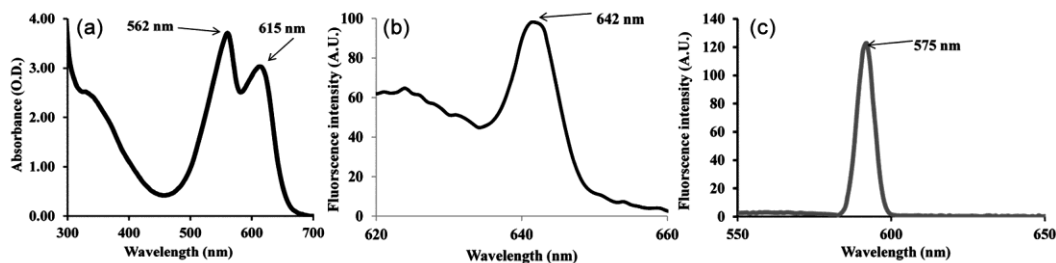
Fig. 4 — Absorption spectrum (A) and Emission spectra of PC (B) and PE (C) of PBP respectively of phytoplankton collected from the river Ganges at Varanasi.
