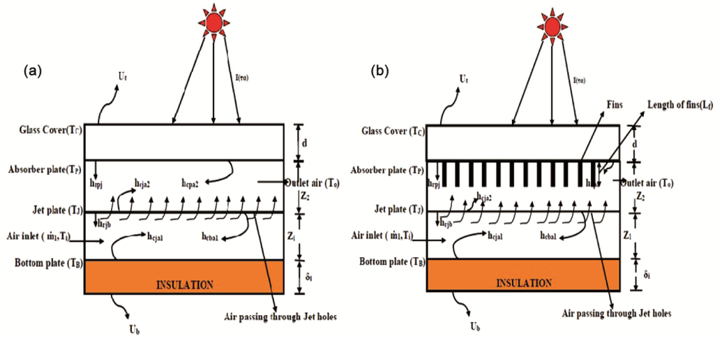
Fig. 1 — (a) Simple impacting air jets SAH (b) impacting air jets-fins
