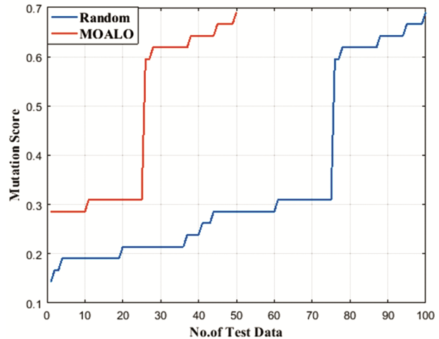
Fig. 4 — Relationships between the mutation score and number of test data
