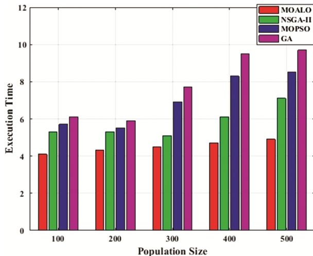
Fig. 5 — Comparison in execution time (sec) of existing systems for different population size (in thousands)
