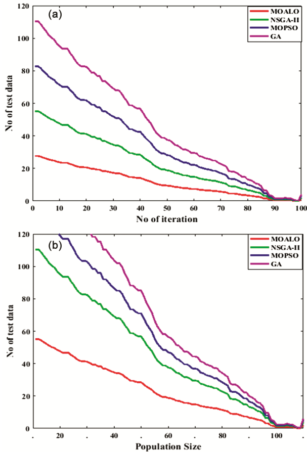
Fig. 2— (a) Relationship between the numbers of test data and the number of iteration and (b), Connection between population size (in thousands) and number of test data
